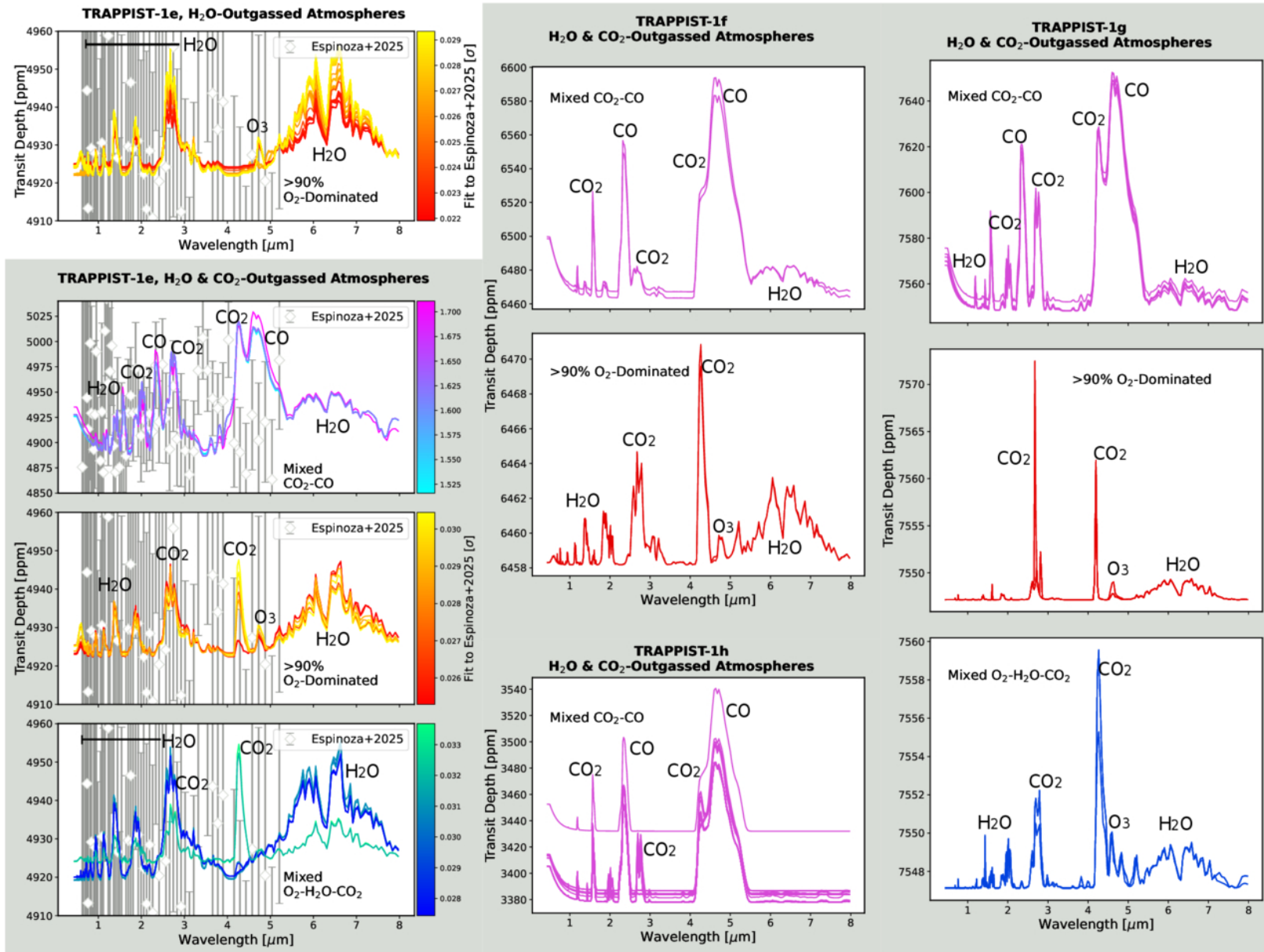
Figure 9. from Megan T. Gialluca et al 2026 Planet. Sci. J. 7 doi:10.3847/PSJ/ae6cef https://dx.doi.org/10.3847/PSJ/ae6cef © 2026. The Author(s). Published by the American Astronomical Society.
