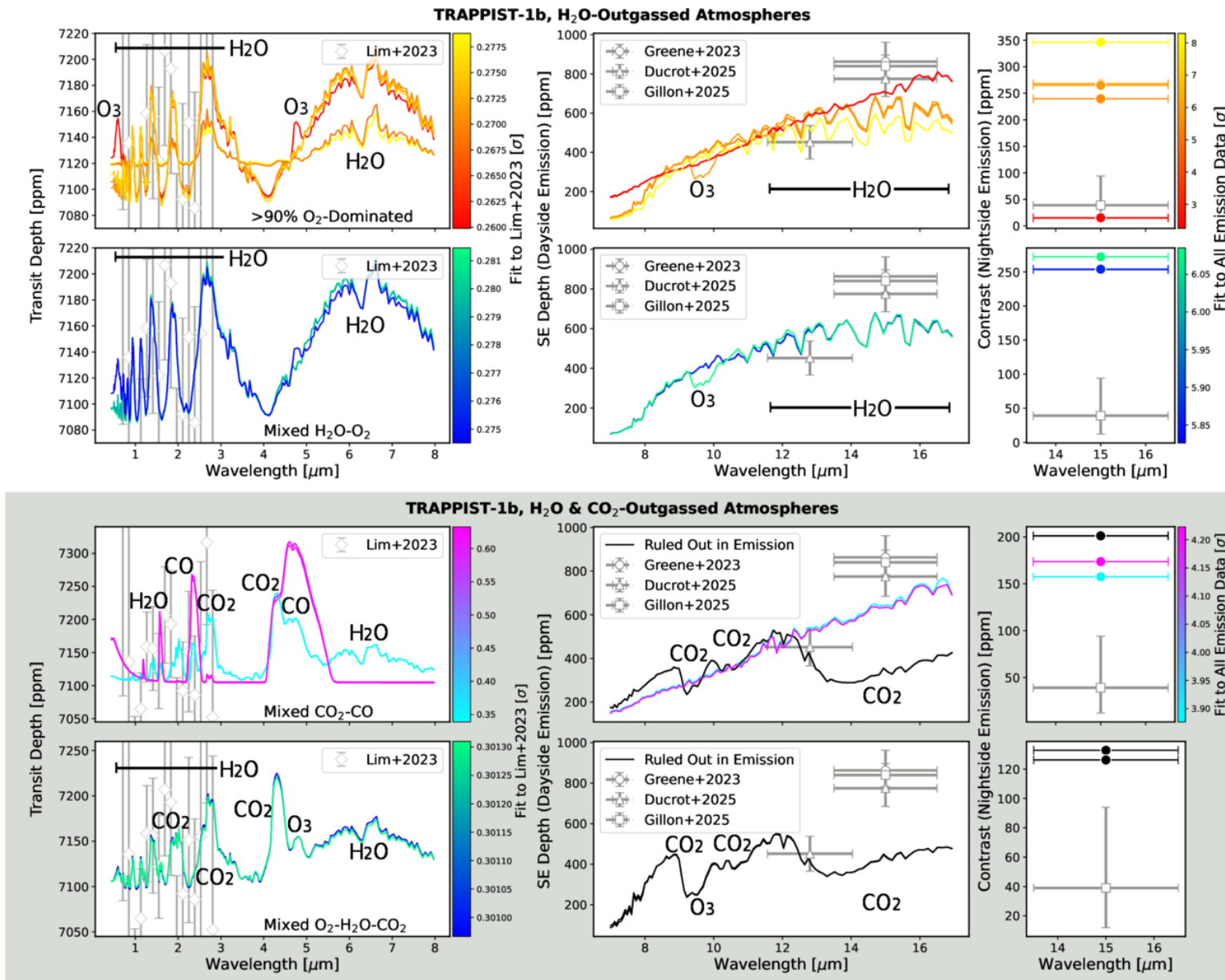
Figure 7. from Megan T. Gialluca et al 2026 Planet. Sci. J. 7 doi:10.3847/PSJ/ae6cef https://dx.doi.org/10.3847/PSJ/ae6cef © 2026. The Author(s). Published by the American Astronomical Society.
