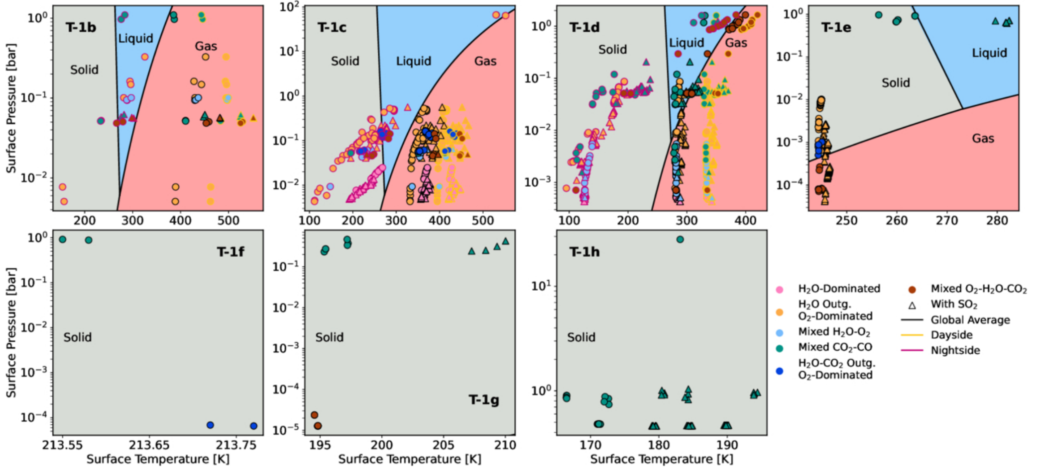
Figure 4. from Megan T. Gialluca et al 2026 Planet. Sci. J. 7 doi:10.3847/PSJ/ae6cef https://dx.doi.org/10.3847/PSJ/ae6cef © 2026. The Author(s). Published by the American Astronomical Society.
