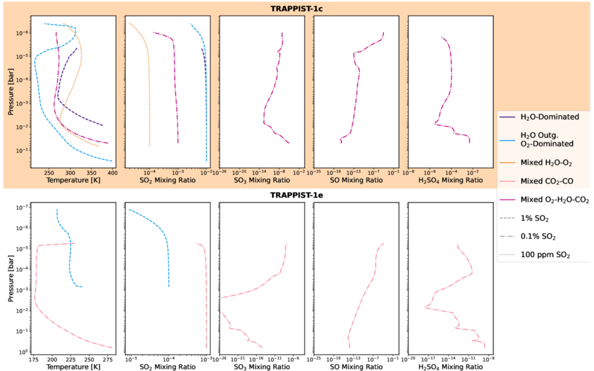
Figure 3. from Megan T. Gialluca et al 2026 Planet. Sci. J. 7 doi:10.3847/PSJ/ae6cef https://dx.doi.org/10.3847/PSJ/ae6cef © 2026. The Author(s). Published by the American Astronomical Society.
