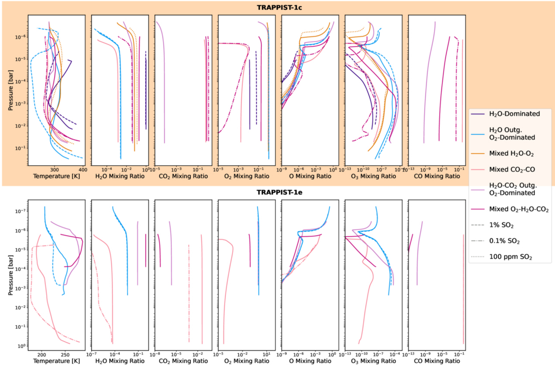
Figure 2. from Megan T. Gialluca et al 2026 Planet. Sci. J. 7 doi:10.3847/PSJ/ae6cef https://dx.doi.org/10.3847/PSJ/ae6cef © 2026. The Author(s). Published by the American Astronomical Society.
