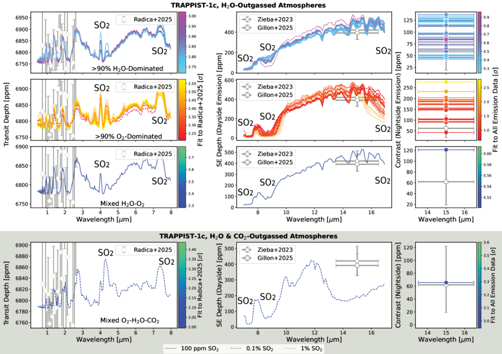
Figure 11. from Megan T. Gialluca et al 2026 Planet. Sci. J. 7 doi:10.3847/PSJ/ae6cef https://dx.doi.org/10.3847/PSJ/ae6cef © 2026. The Author(s). Published by the American Astronomical Society.
