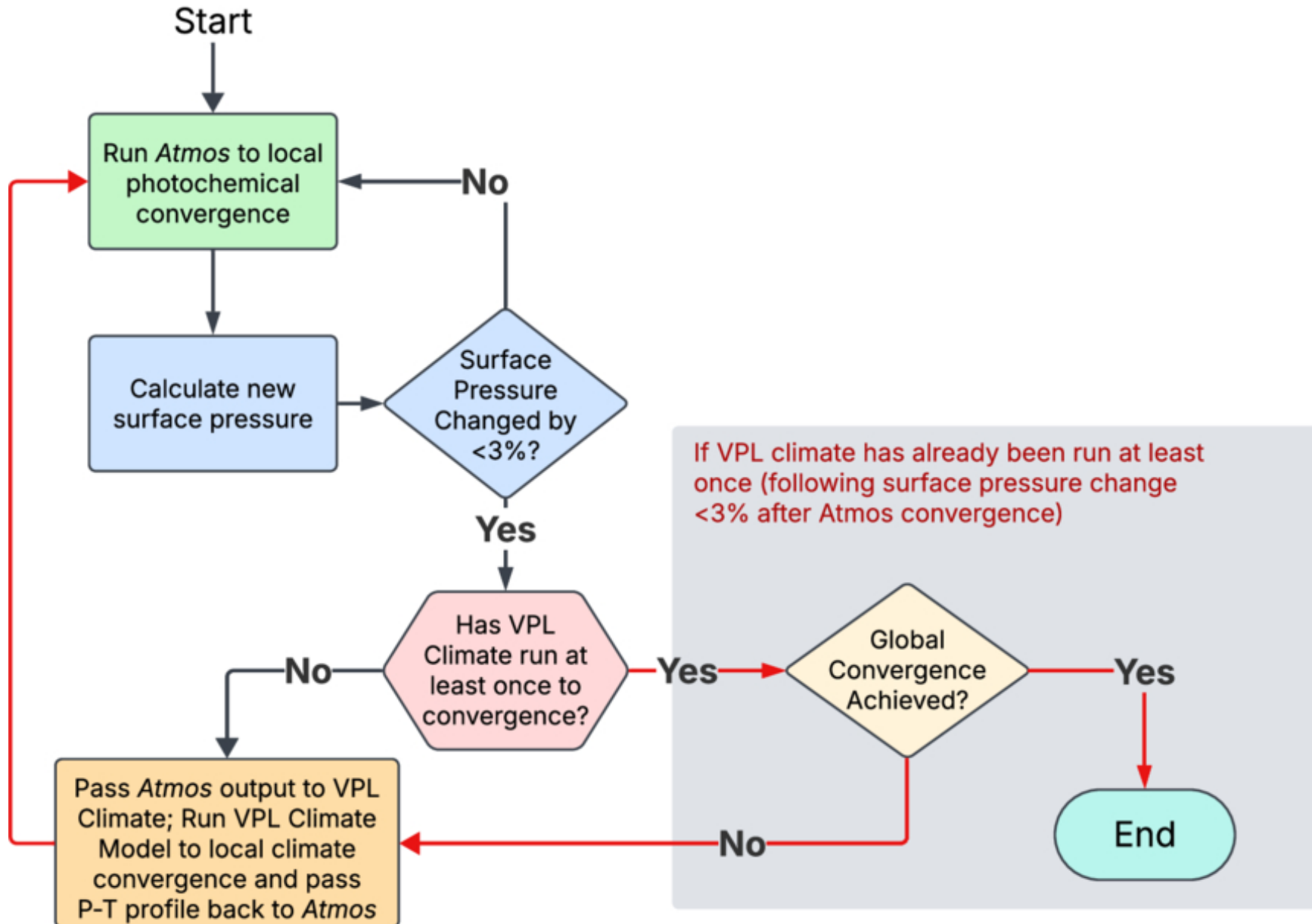
Figure 1. from Megan T. Gialluca et al 2026 Planet. Sci. J. 7 doi:10.3847/PSJ/ae6cef https://dx.doi.org/10.3847/PSJ/ae6cef © 2026. The Author(s). Published by the American Astronomical Society.
