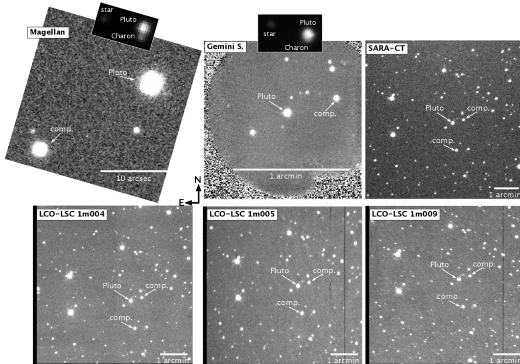
Figure 9. from Amanda A. Sickafoose et al 2026 Planet. Sci. J. 7 doi:10.3847/PSJ/ae6cdd https://dx.doi.org/10.3847/PSJ/ae6cdd © 2026. The Author(s). Published by the American Astronomical Society.
