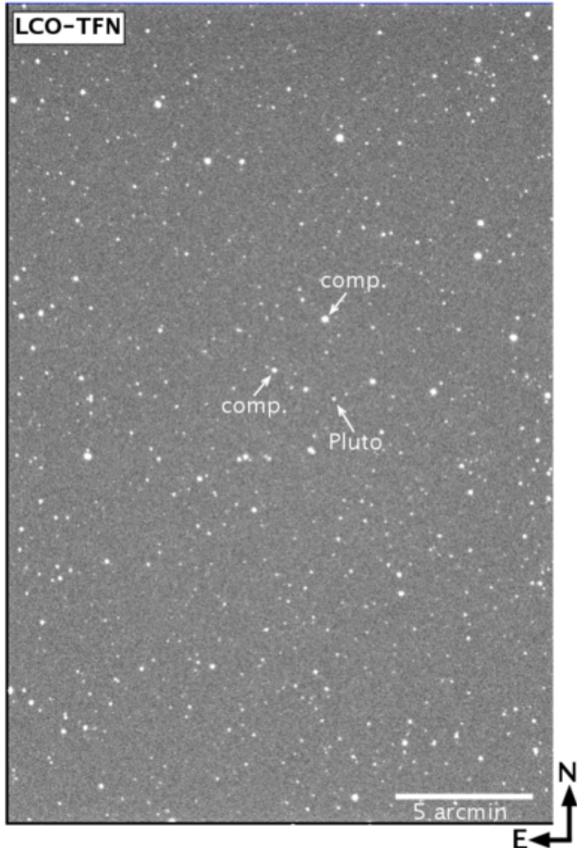
Figure 8. from Amanda A. Sickafoose et al 2026 Planet. Sci. J. 7 doi:10.3847/PSJ/ae6cdd https://dx.doi.org/10.3847/PSJ/ae6cdd © 2026. The Author(s). Published by the American Astronomical Society.
