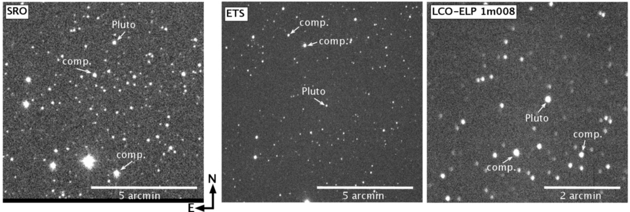
Figure 5. from Amanda A. Sickafoose et al 2026 Planet. Sci. J. 7 doi:10.3847/PSJ/ae6cdd https://dx.doi.org/10.3847/PSJ/ae6cdd © 2026. The Author(s). Published by the American Astronomical Society.
