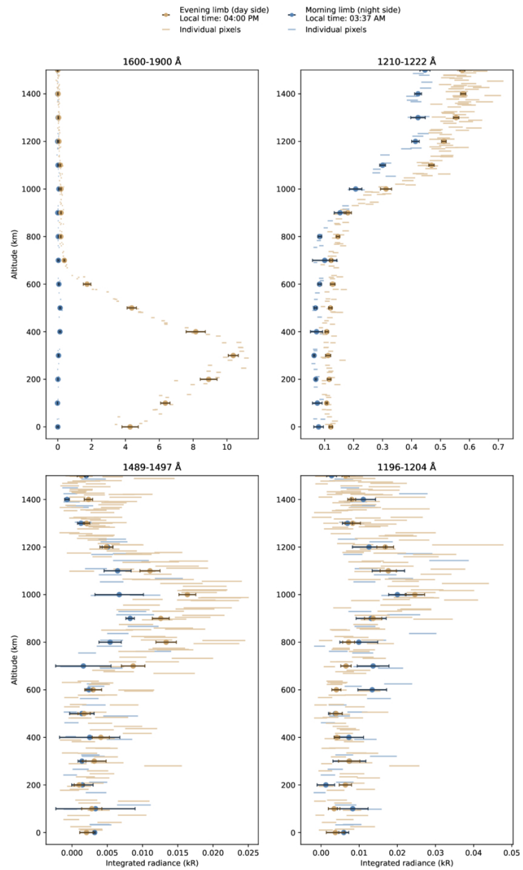
Figure 9. from Nathan Le Guennic et al 2026 Planet. Sci. J. 7 doi:10.3847/PSJ/ae6c24 https://dx.doi.org/10.3847/PSJ/ae6c24 © 2026. The Author(s). Published by the American Astronomical Society.
