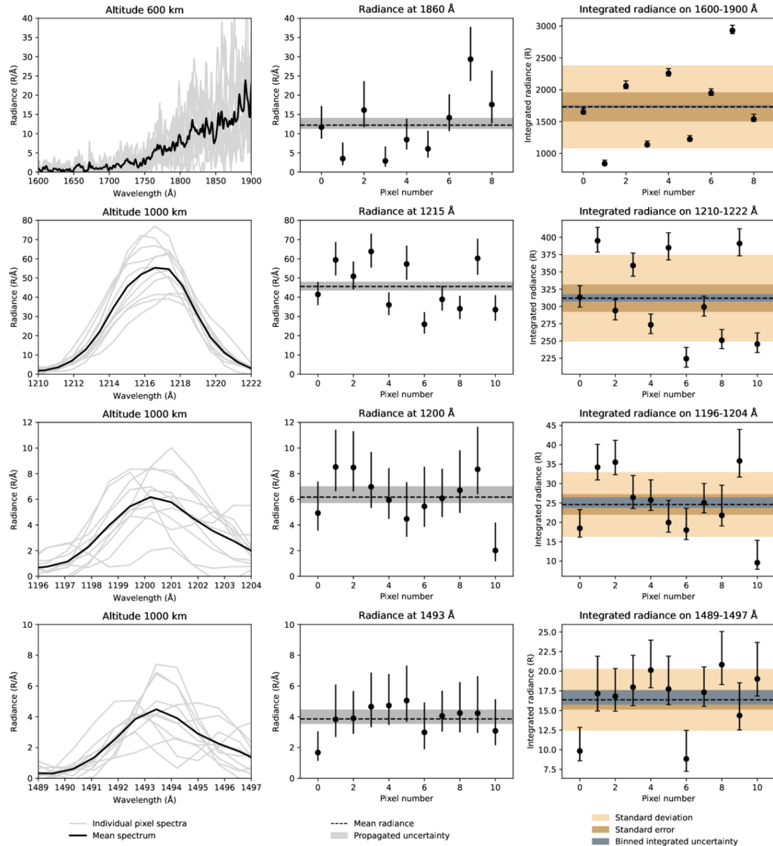
Figure 8. from Nathan Le Guennic et al 2026 Planet. Sci. J. 7 doi:10.3847/PSJ/ae6c24 https://dx.doi.org/10.3847/PSJ/ae6c24 © 2026. The Author(s). Published by the American Astronomical Society.
