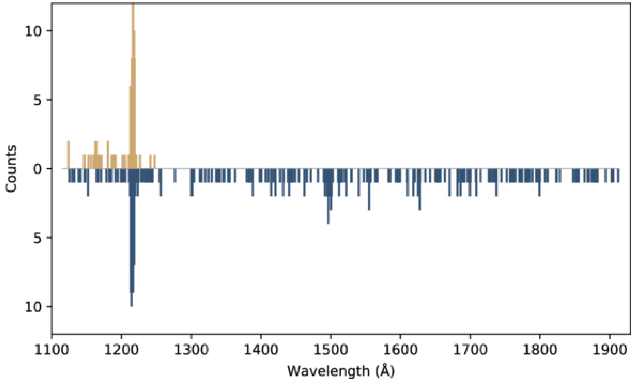
Figure 5. from Nathan Le Guennic et al 2026 Planet. Sci. J. 7 doi:10.3847/PSJ/ae6c24 https://dx.doi.org/10.3847/PSJ/ae6c24 © 2026. The Author(s). Published by the American Astronomical Society.
