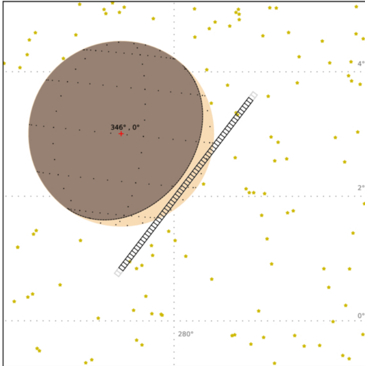
Figure 1. from Nathan Le Guennic et al 2026 Planet. Sci. J. 7 doi:10.3847/PSJ/ae6c24 https://dx.doi.org/10.3847/PSJ/ae6c24 © 2026. The Author(s). Published by the American Astronomical Society.
