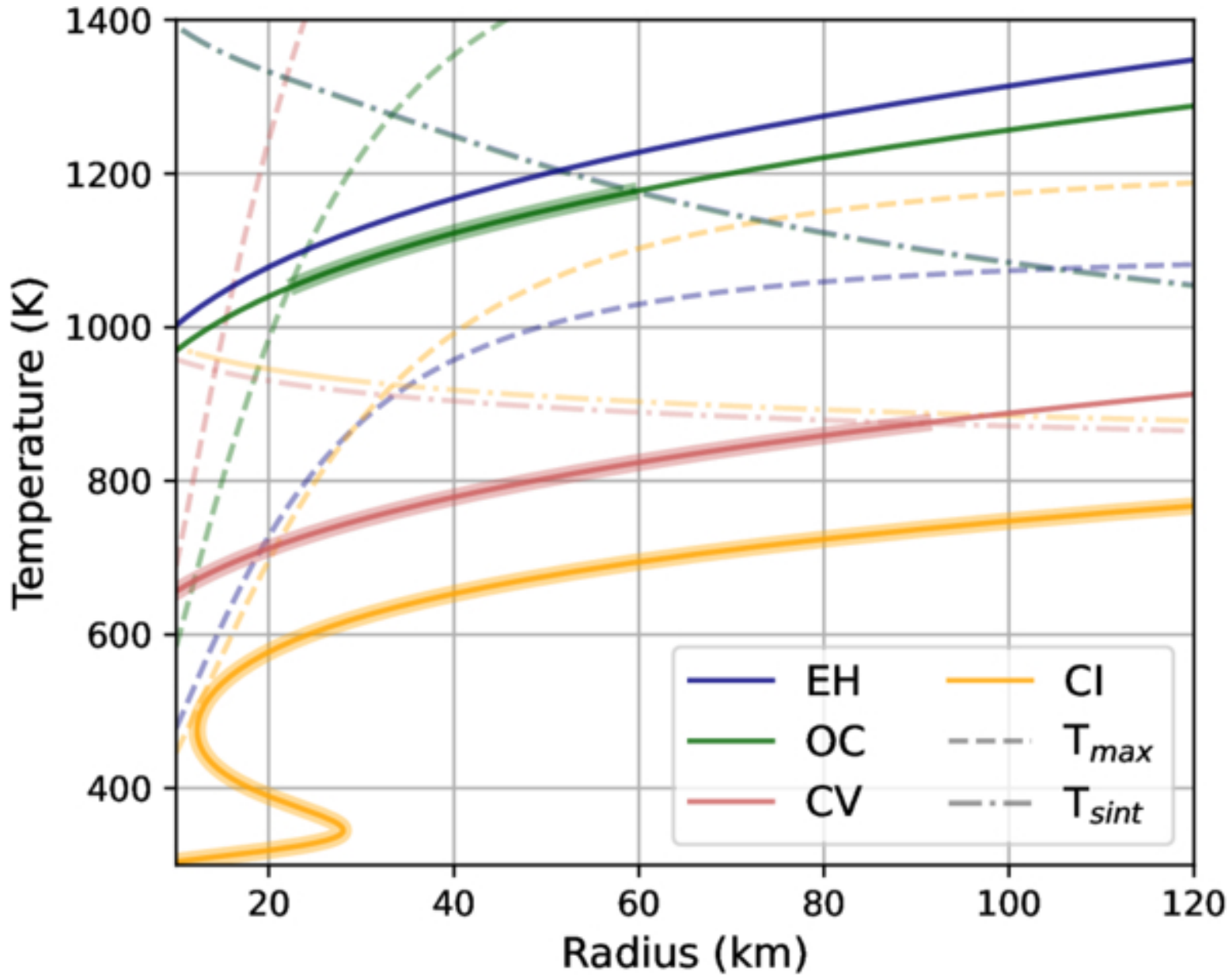
Figure 9. from Bo Peng et al 2026 Planet. Sci. J. 7 doi:10.3847/PSJ/ae6c21 https://dx.doi.org/10.3847/PSJ/ae6c21 © 2026. The Author(s). Published by the American Astronomical Society.
