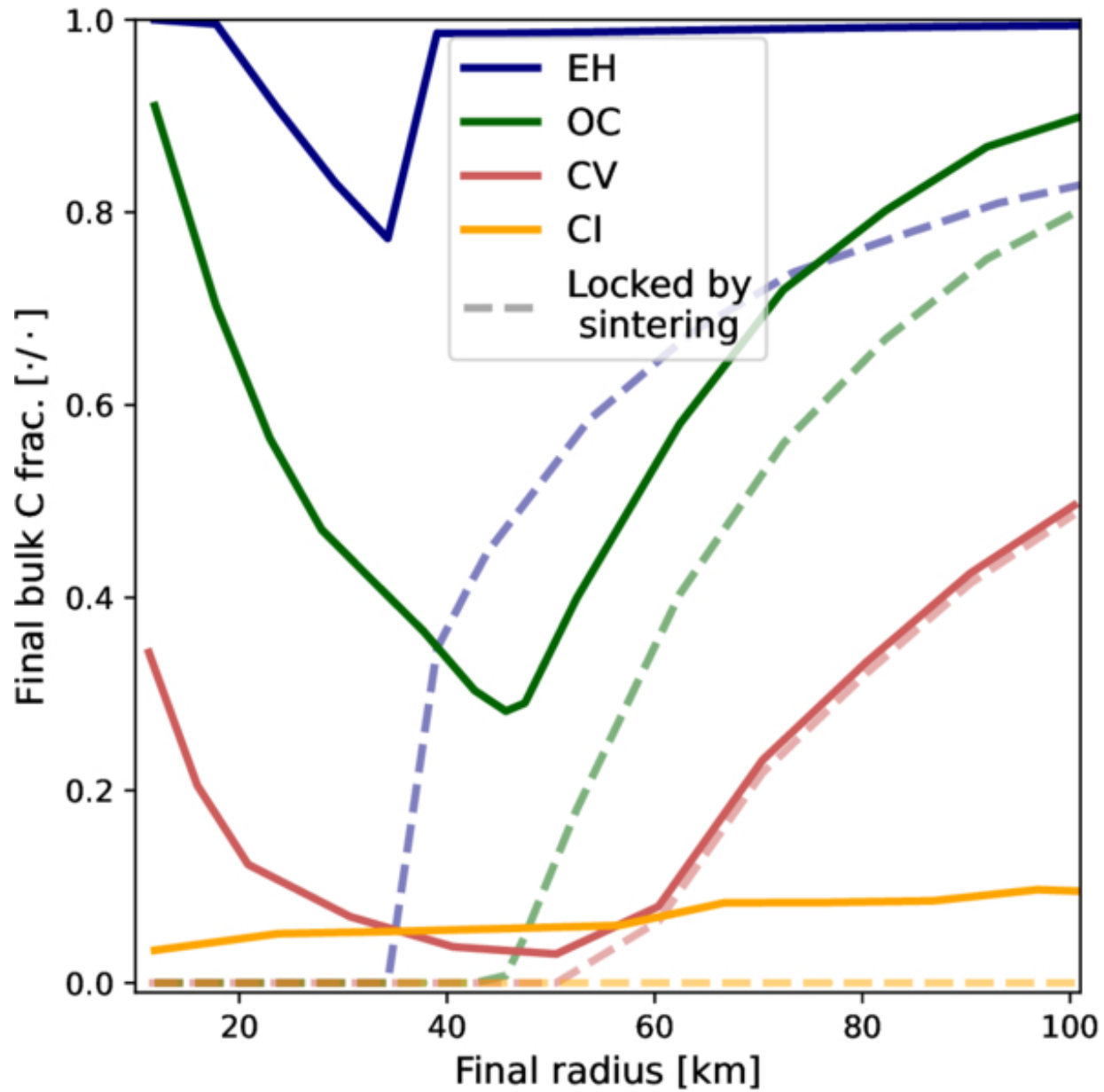
Figure 3. from Bo Peng et al 2026 Planet. Sci. J. 7 doi:10.3847/PSJ/ae6c21 https://dx.doi.org/10.3847/PSJ/ae6c21 © 2026. The Author(s). Published by the American Astronomical Society.
