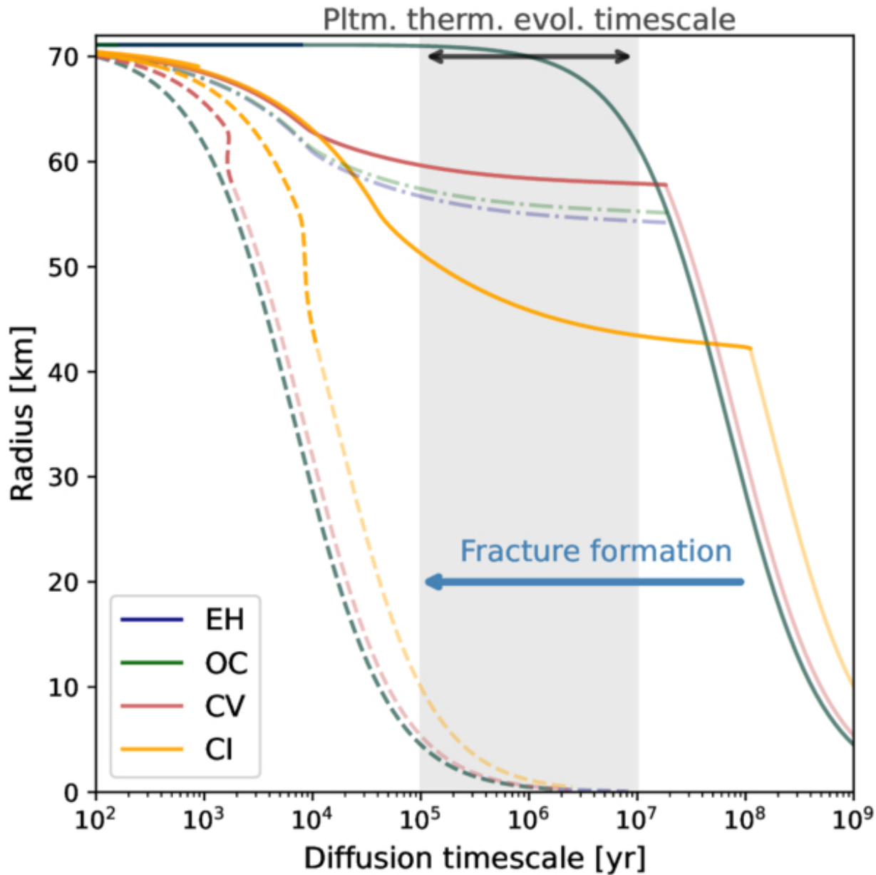
Figure 11. from Bo Peng et al 2026 Planet. Sci. J. 7 doi:10.3847/PSJ/ae6c21 https://dx.doi.org/10.3847/PSJ/ae6c21 © 2026. The Author(s). Published by the American Astronomical Society.
