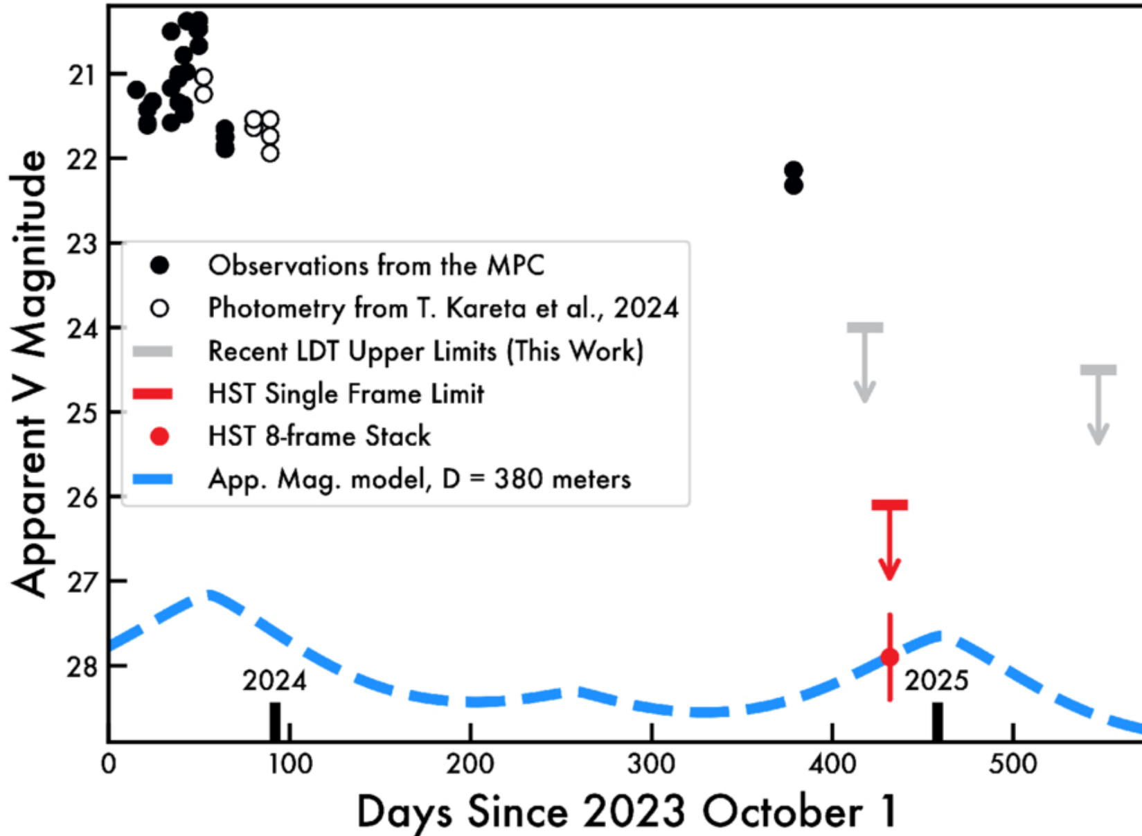
Figure 2. from John W. Noonan and Theodore Kareta 2026 Planet. Sci. J. 7 doi:10.3847/PSJ/ae6c1d https://dx.doi.org/10.3847/PSJ/ae6c1d © 2026. The Author(s). Published by the American Astronomical Society.
