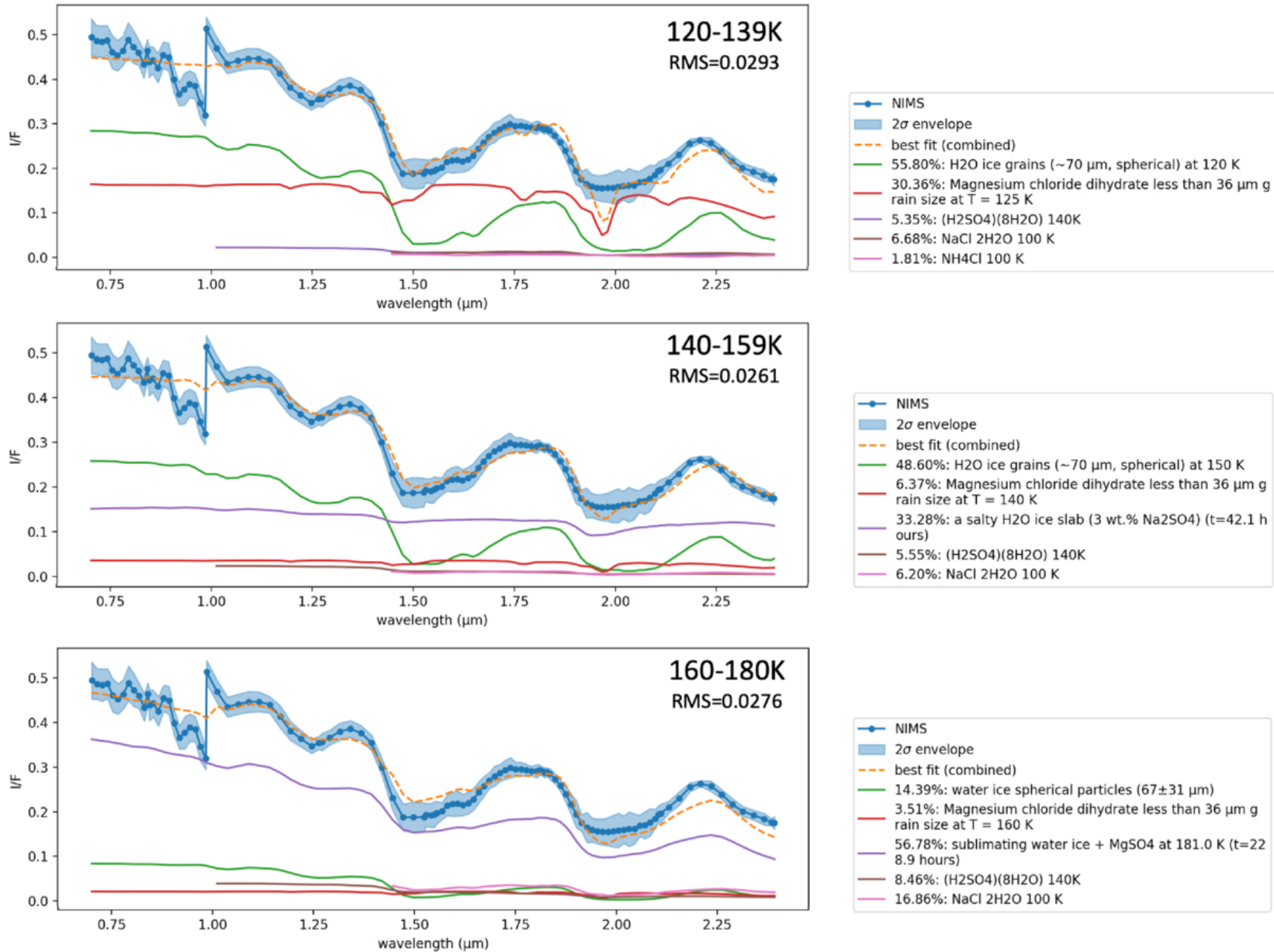
Figure 9. from Anezina Solomonidou et al 2026 Planet. Sci. J. 7 doi:10.3847/PSJ/ae69cd https://dx.doi.org/10.3847/PSJ/ae69cd © 2026 The Author(s). Published by the American Astronomical Society.
