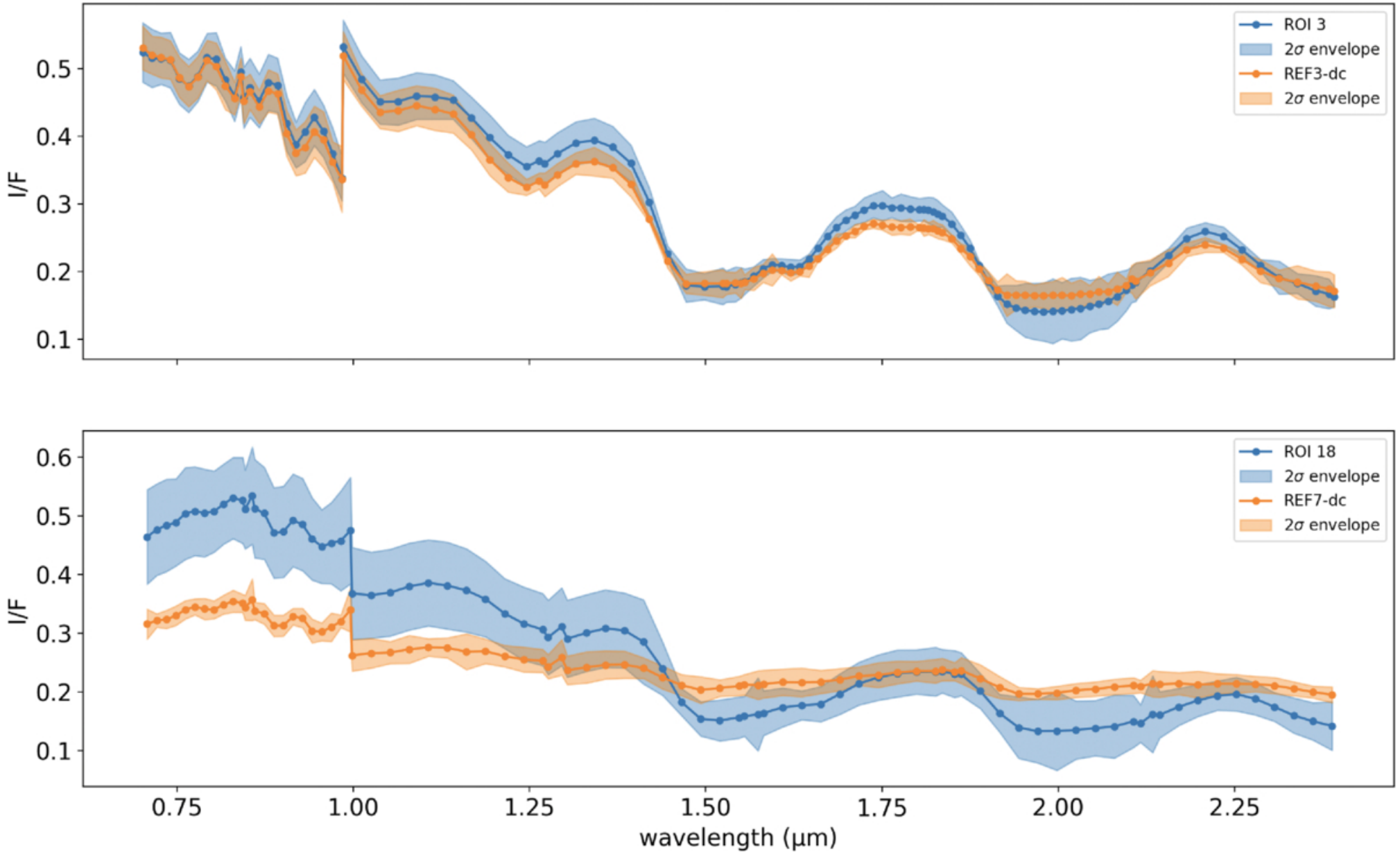
Figure 8. from Anezina Solomonidou et al 2026 Planet. Sci. J. 7 doi:10.3847/PSJ/ae69cd https://dx.doi.org/10.3847/PSJ/ae69cd © 2026 The Author(s). Published by the American Astronomical Society.
