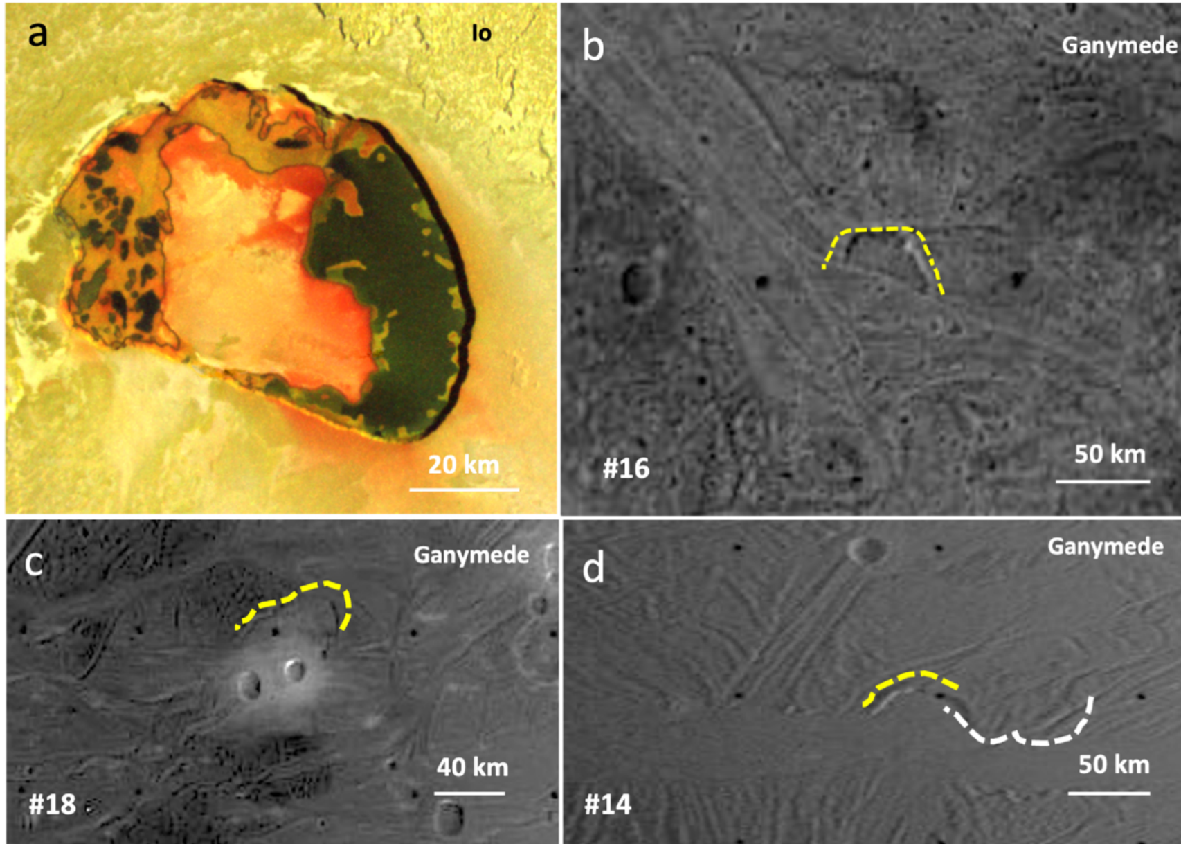
Figure 5. from Anezina Solomonidou et al 2026 Planet. Sci. J. 7 doi:10.3847/PSJ/ae69cd https://dx.doi.org/10.3847/PSJ/ae69cd © 2026 The Author(s). Published by the American Astronomical Society.
