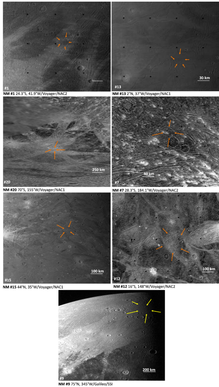
Figure 3. from Anezina Solomonidou et al 2026 Planet. Sci. J. 7 doi:10.3847/PSJ/ae69cd https://dx.doi.org/10.3847/PSJ/ae69cd © 2026 The Author(s). Published by the American Astronomical Society.
