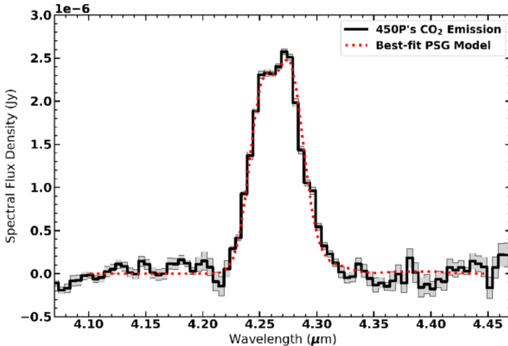
Figure 7. from Charles A. Schambeau et al 2026 Planet. Sci. J. 7 doi:10.3847/PSJ/ae685c https://dx.doi.org/10.3847/PSJ/ae685c © 2026. The Author(s). Published by the American Astronomical Society.
