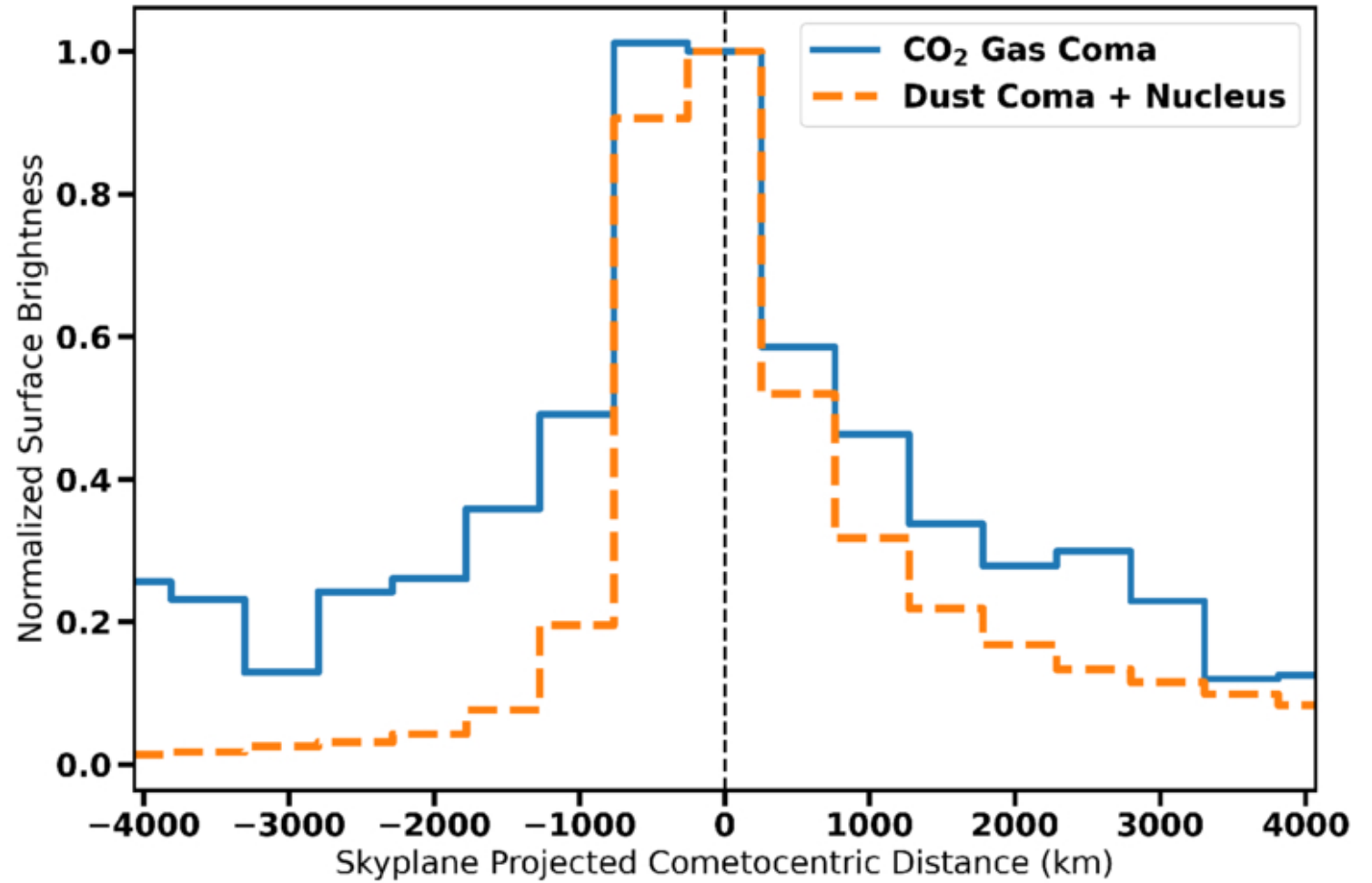
Figure 6. from Charles A. Schambeau et al 2026 Planet. Sci. J. 7 doi:10.3847/PSJ/ae685c https://dx.doi.org/10.3847/PSJ/ae685c © 2026. The Author(s). Published by the American Astronomical Society.
