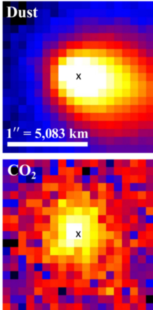
Figure 6. from Charles A. Schambeau et al 2026 Planet. Sci. J. 7 doi:10.3847/PSJ/ae685c https://dx.doi.org/10.3847/PSJ/ae685c © 2026. The Author(s). Published by the American Astronomical Society.
