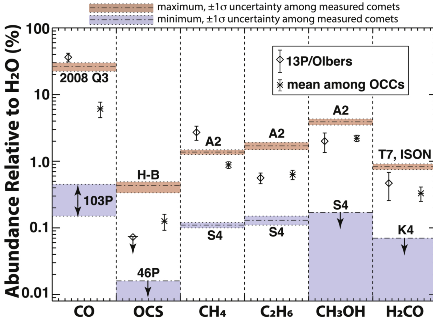
Figure 6. from Michael A. DiSanti et al 2026 Planet. Sci. J. 7 doi:10.3847/PSJ/ae66fb https://dx.doi.org/10.3847/PSJ/ae66fb © 2026. The Author(s). Published by the American Astronomical Society.
