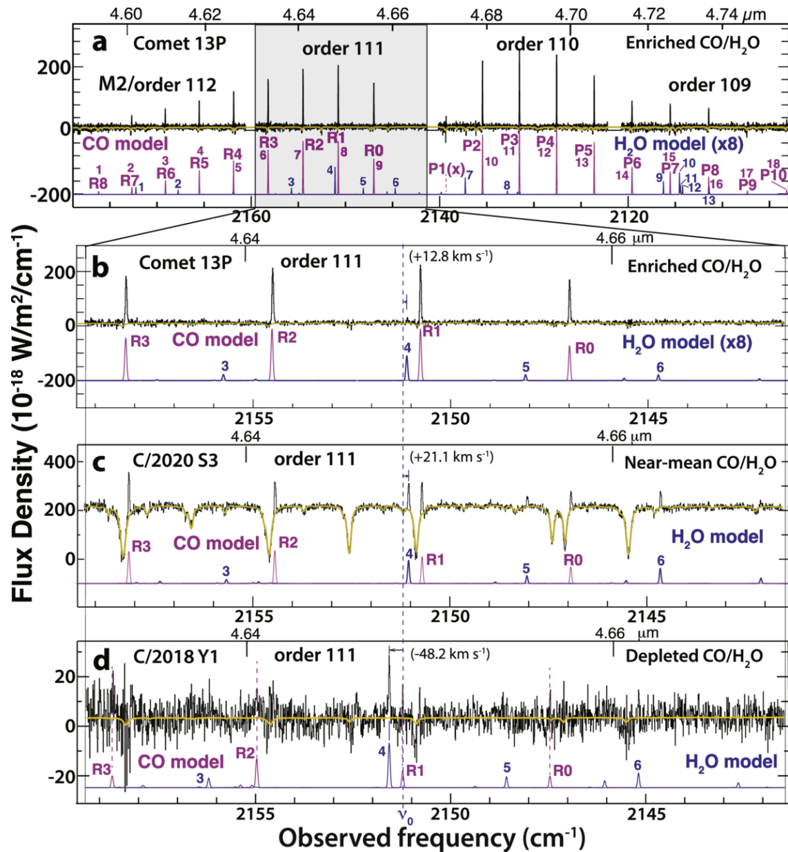
Figure 2. from Michael A. DiSanti et al 2026 Planet. Sci. J. 7 doi:10.3847/PSJ/ae66fb https://dx.doi.org/10.3847/PSJ/ae66fb © 2026. The Author(s). Published by the American Astronomical Society.
