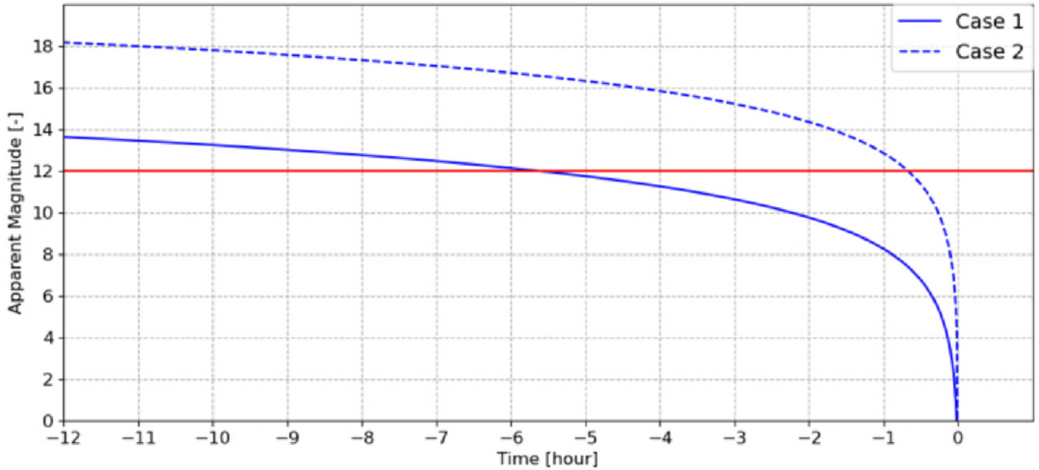
Figure 7. from Kaho Nakagawa et al 2026 Planet. Sci. J. 7 doi:10.3847/PSJ/ae66f2 https://dx.doi.org/10.3847/PSJ/ae66f2 © 2026. The Author(s). Published by the American Astronomical Society.
