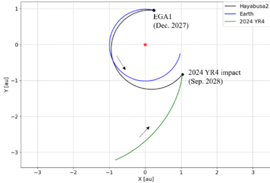
Figure 5. from Kaho Nakagawa et al 2026 Planet. Sci. J. 7 doi:10.3847/PSJ/ae66f2 https://dx.doi.org/10.3847/PSJ/ae66f2 © 2026. The Author(s). Published by the American Astronomical Society.
