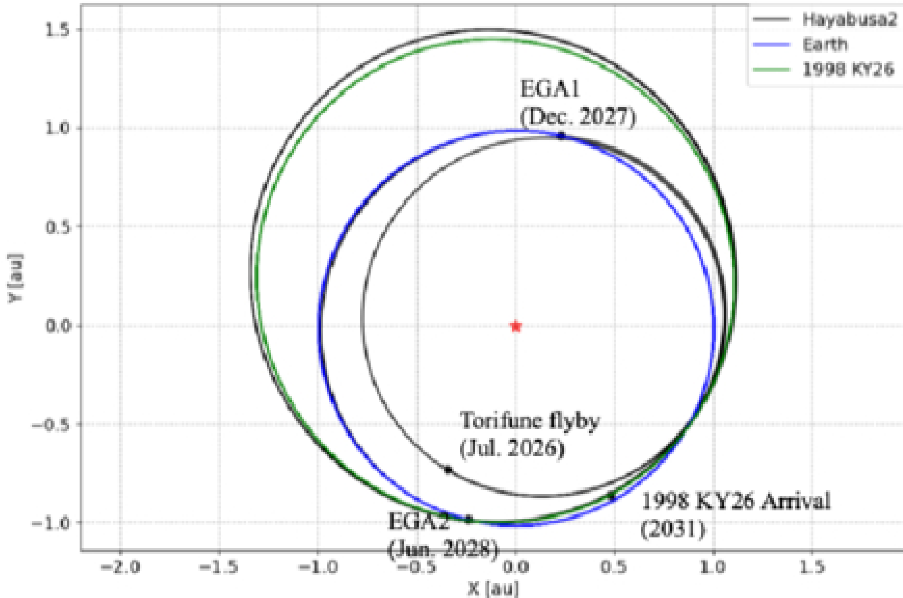
Figure 4. from Kaho Nakagawa et al 2026 Planet. Sci. J. 7 doi:10.3847/PSJ/ae66f2 https://dx.doi.org/10.3847/PSJ/ae66f2 © 2026. The Author(s). Published by the American Astronomical Society.
