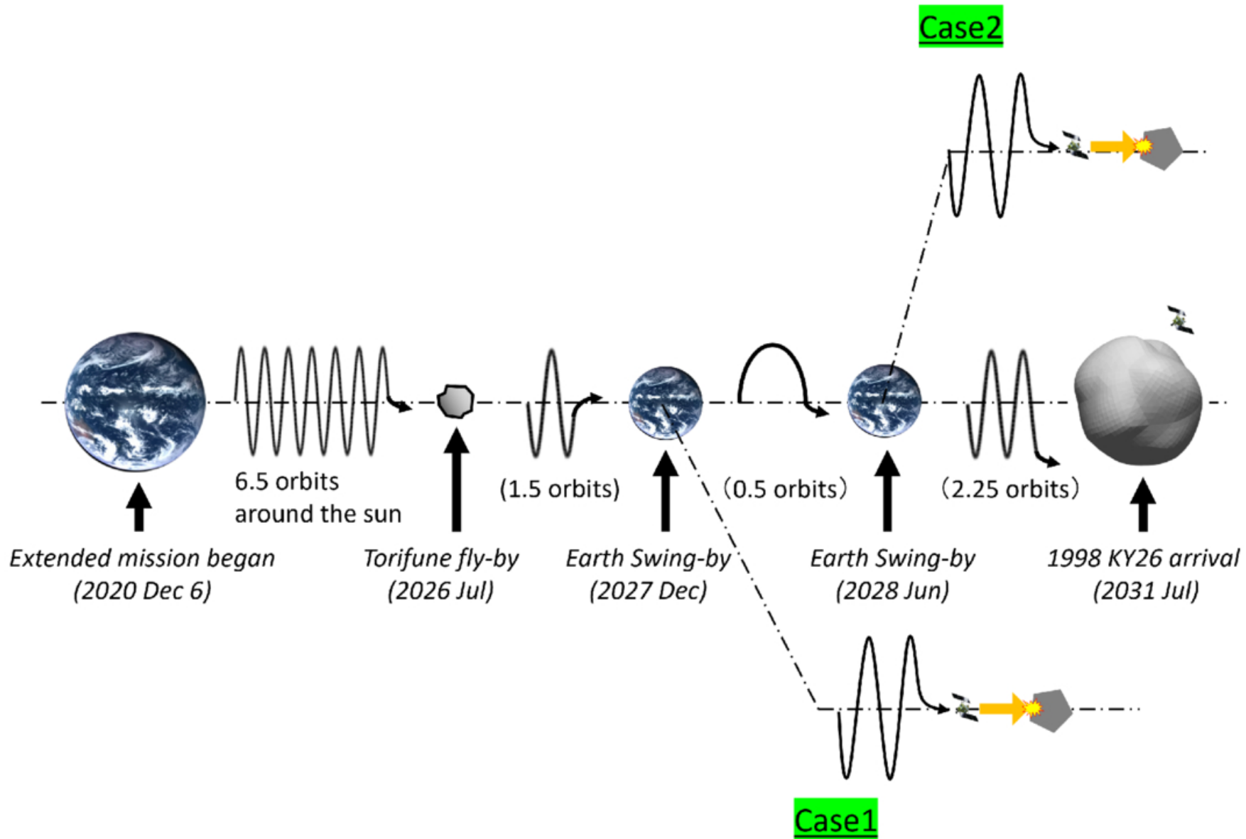
Figure 3. from Kaho Nakagawa et al 2026 Planet. Sci. J. 7 doi:10.3847/PSJ/ae66f2 https://dx.doi.org/10.3847/PSJ/ae66f2 © 2026. The Author(s). Published by the American Astronomical Society.
