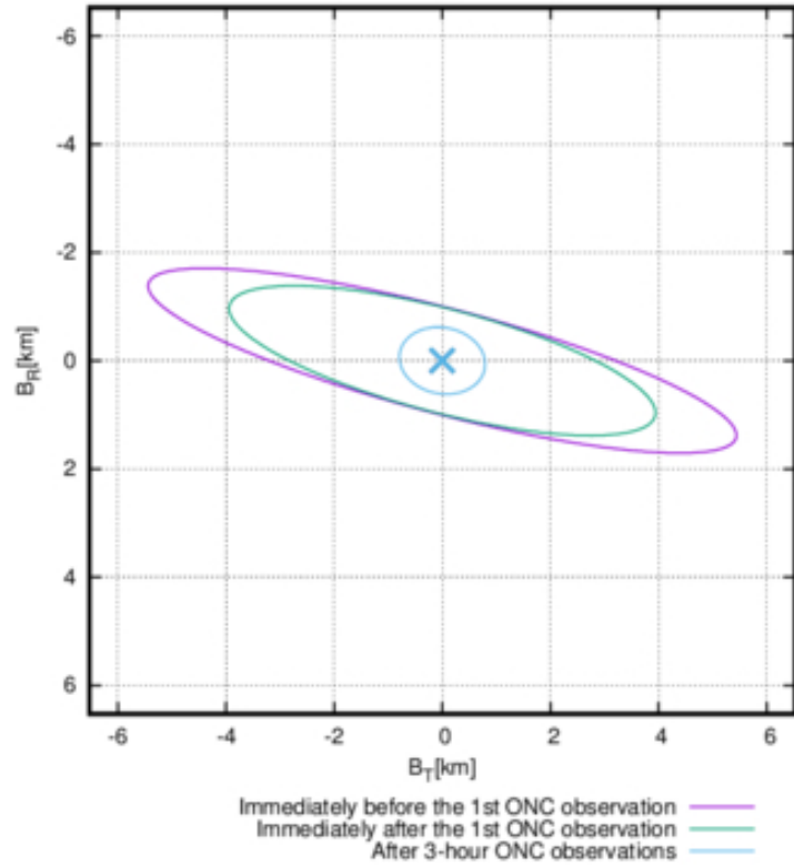
Figure 14. from Kaho Nakagawa et al 2026 Planet. Sci. J. 7 doi:10.3847/PSJ/ae66f2 https://dx.doi.org/10.3847/PSJ/ae66f2 © 2026. The Author(s). Published by the American Astronomical Society.
