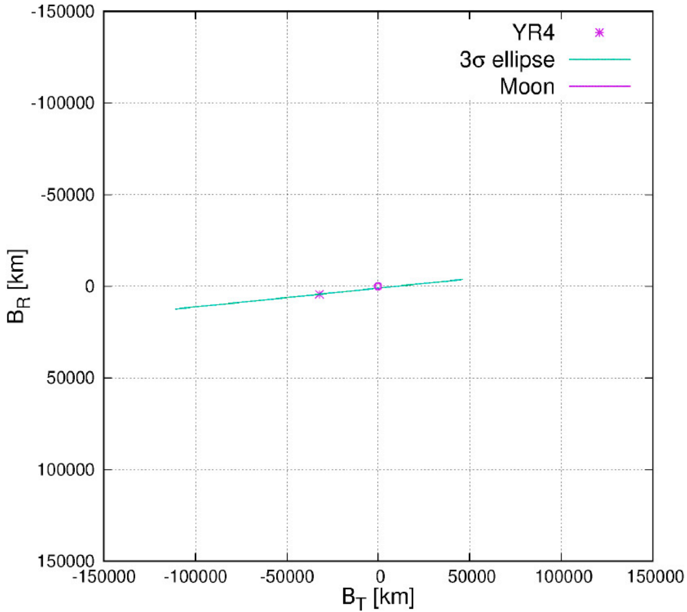
Figure 10. from Kaho Nakagawa et al 2026 Planet. Sci. J. 7 doi:10.3847/PSJ/ae66f2 https://dx.doi.org/10.3847/PSJ/ae66f2 © 2026. The Author(s). Published by the American Astronomical Society.
