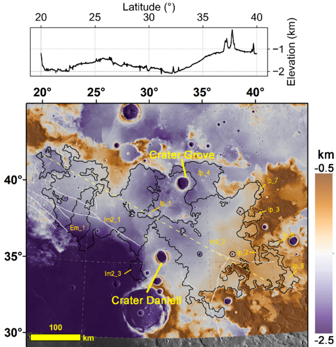
Figure 2. from Yihao Chen et al 2026 Planet. Sci. J. 7 doi:10.3847/PSJ/ae66e4 https://dx.doi.org/10.3847/PSJ/ae66e4 © 2026. The Author(s). Published by the American Astronomical Society.
