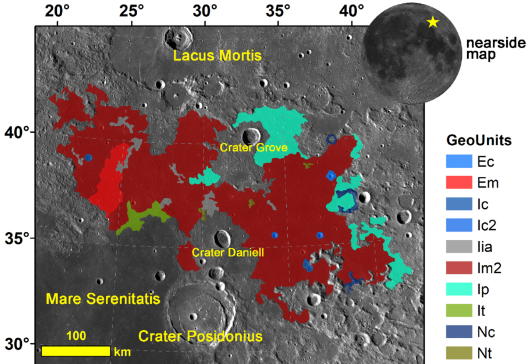
Figure 1. from Yihao Chen et al 2026 Planet. Sci. J. 7 doi:10.3847/PSJ/ae66e4 https://dx.doi.org/10.3847/PSJ/ae66e4 © 2026. The Author(s). Published by the American Astronomical Society.
