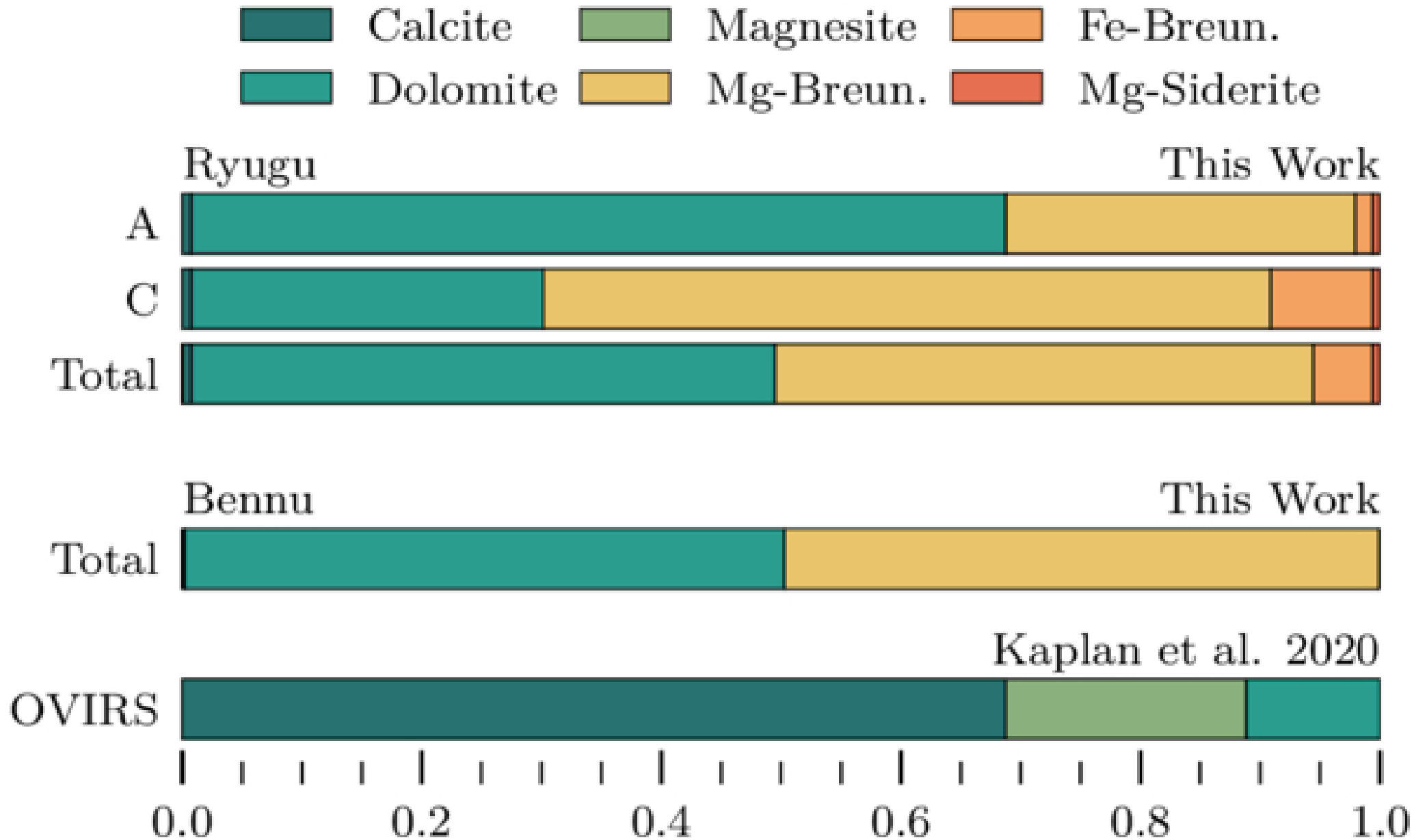
Figure 8. from Max Mahlke et al 2026 Planet. Sci. J. 7 doi:10.3847/PSJ/ae6643 https://dx.doi.org/10.3847/PSJ/ae6643 © 2026. The Author(s). Published by the American Astronomical Society.
