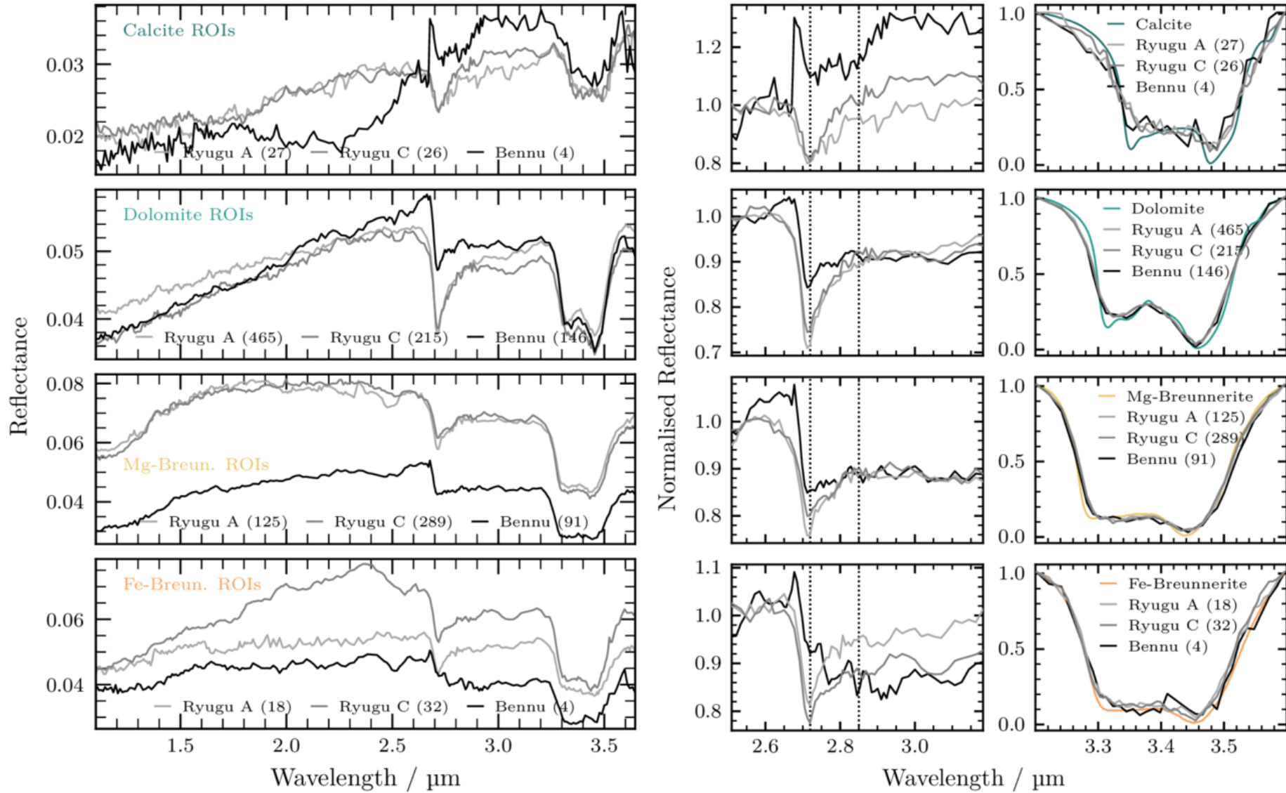
Figure 6. from Max Mahlke et al 2026 Planet. Sci. J. 7 doi:10.3847/PSJ/ae6643 https://dx.doi.org/10.3847/PSJ/ae6643 © 2026. The Author(s). Published by the American Astronomical Society.
