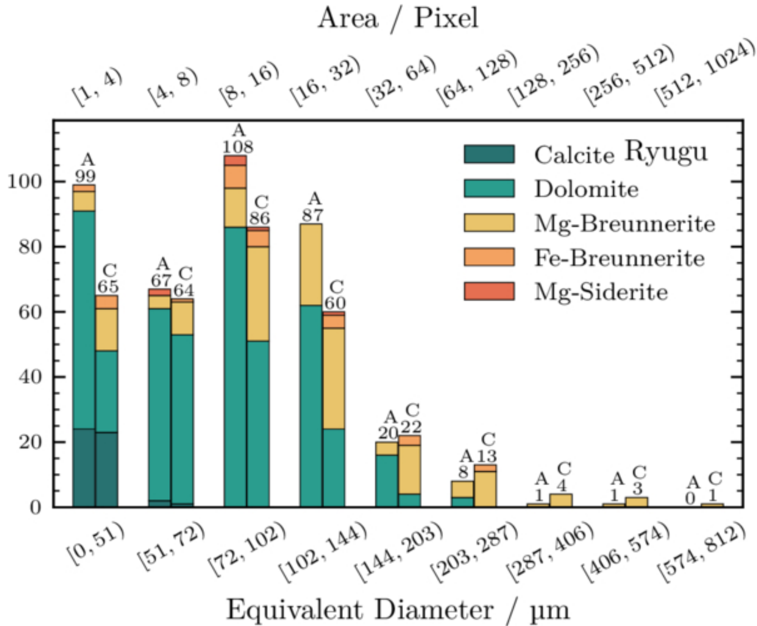
Figure 4. from Max Mahlke et al 2026 Planet. Sci. J. 7 doi:10.3847/PSJ/ae6643 https://dx.doi.org/10.3847/PSJ/ae6643 © 2026. The Author(s). Published by the American Astronomical Society.
