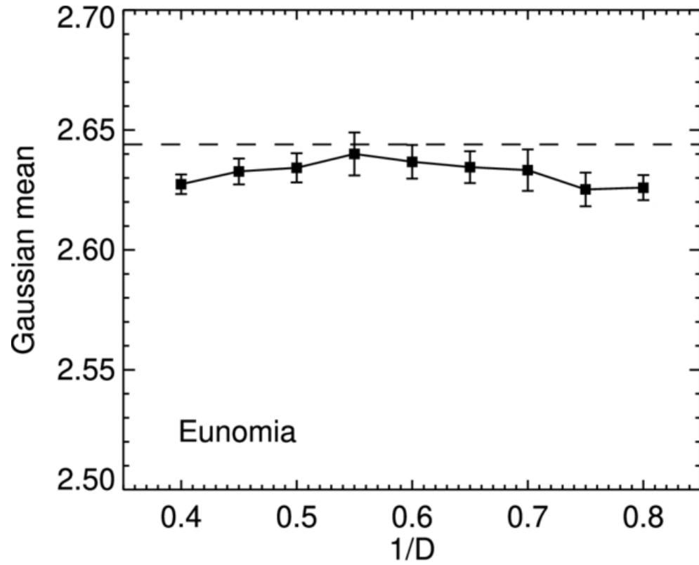
Figure 13. from Stanley F. Dermott et al 2026 Planet. Sci. J. 7 doi:10.3847/PSJ/ae6501 https://dx.doi.org/10.3847/PSJ/ae6501 © 2026. The Author(s). Published by the American Astronomical Society.
