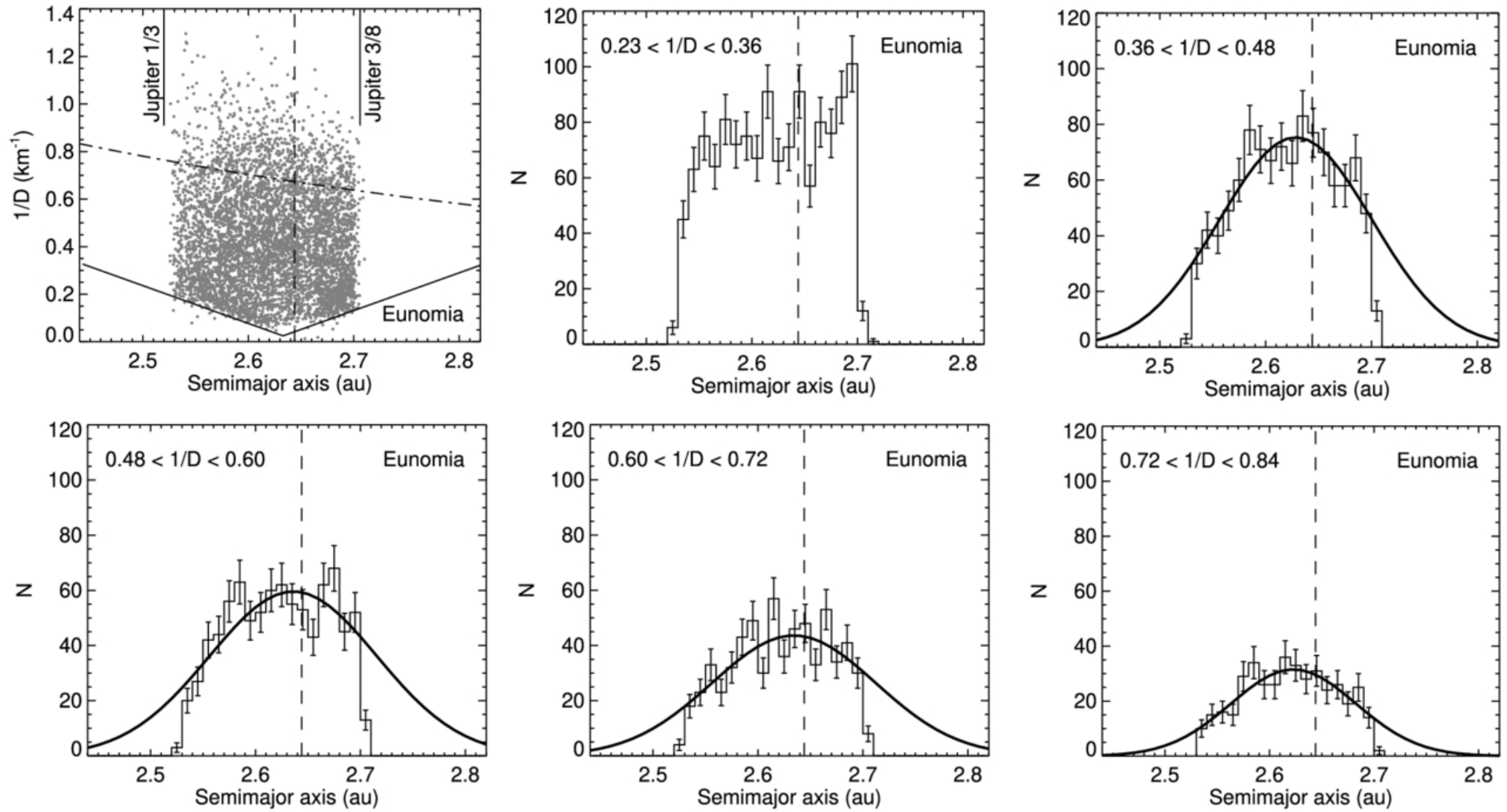
Figure 12. from Stanley F. Dermott et al 2026 Planet. Sci. J. 7 doi:10.3847/PSJ/ae6501 https://dx.doi.org/10.3847/PSJ/ae6501 © 2026. The Author(s). Published by the American Astronomical Society.
