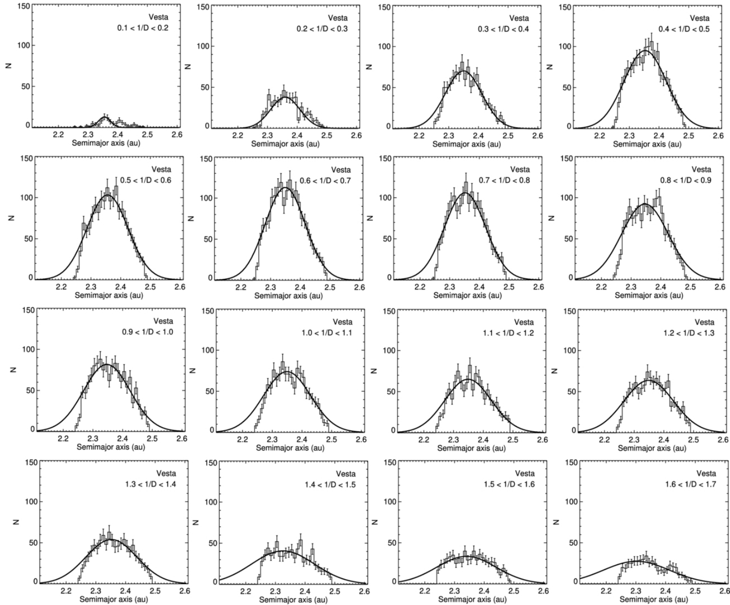
Figure 10. from Stanley F. Dermott et al 2026 Planet. Sci. J. 7 doi:10.3847/PSJ/ae6501 https://dx.doi.org/10.3847/PSJ/ae6501 © 2026. The Author(s). Published by the American Astronomical Society.
