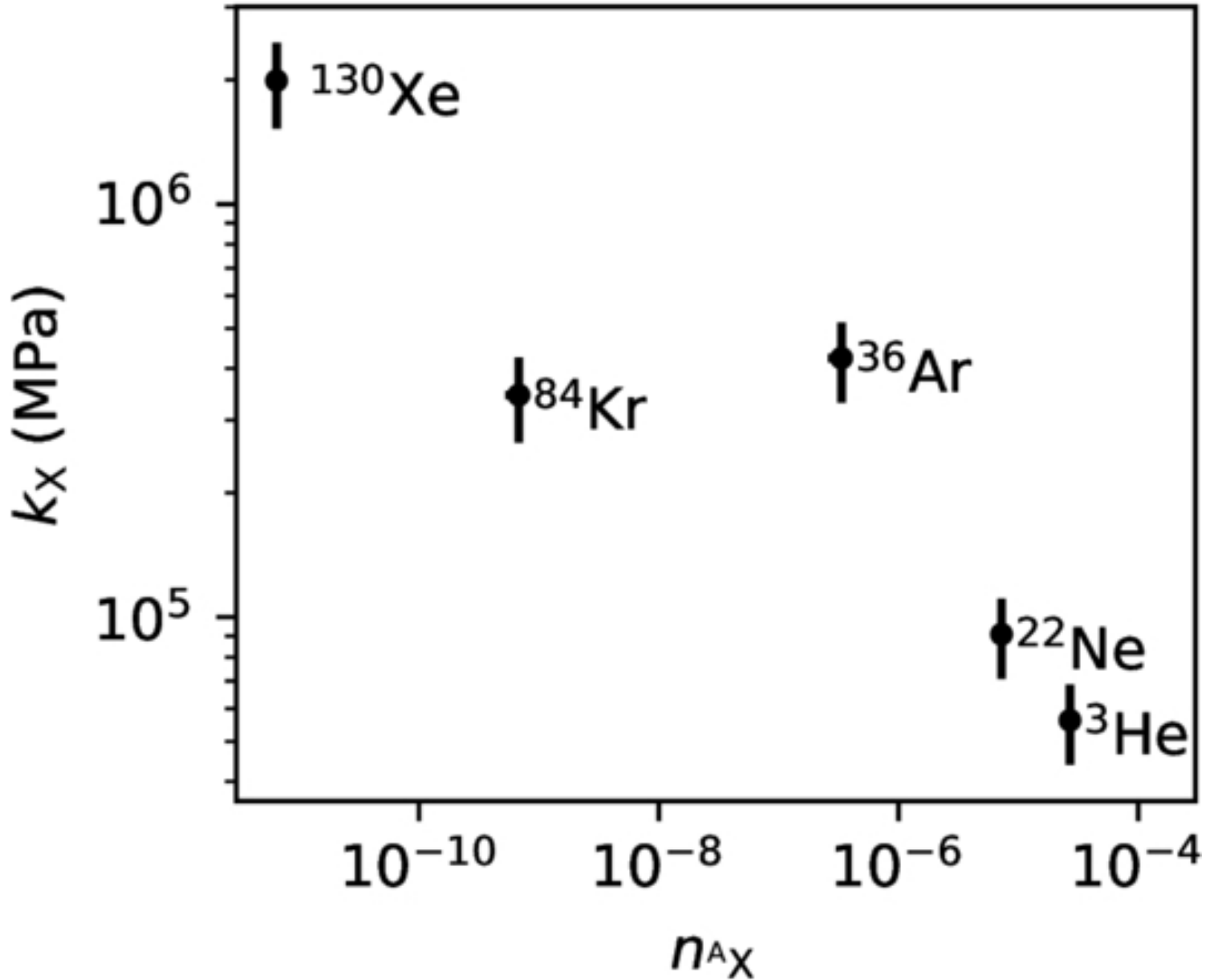
Figure 7. from Vincent Savignac and Eve J. Lee 2026 Planet. Sci. J. 7 doi:10.3847/PSJ/ae64f7 https://dx.doi.org/10.3847/PSJ/ae64f7 © 2026. The Author(s). Published by the American Astronomical Society.
