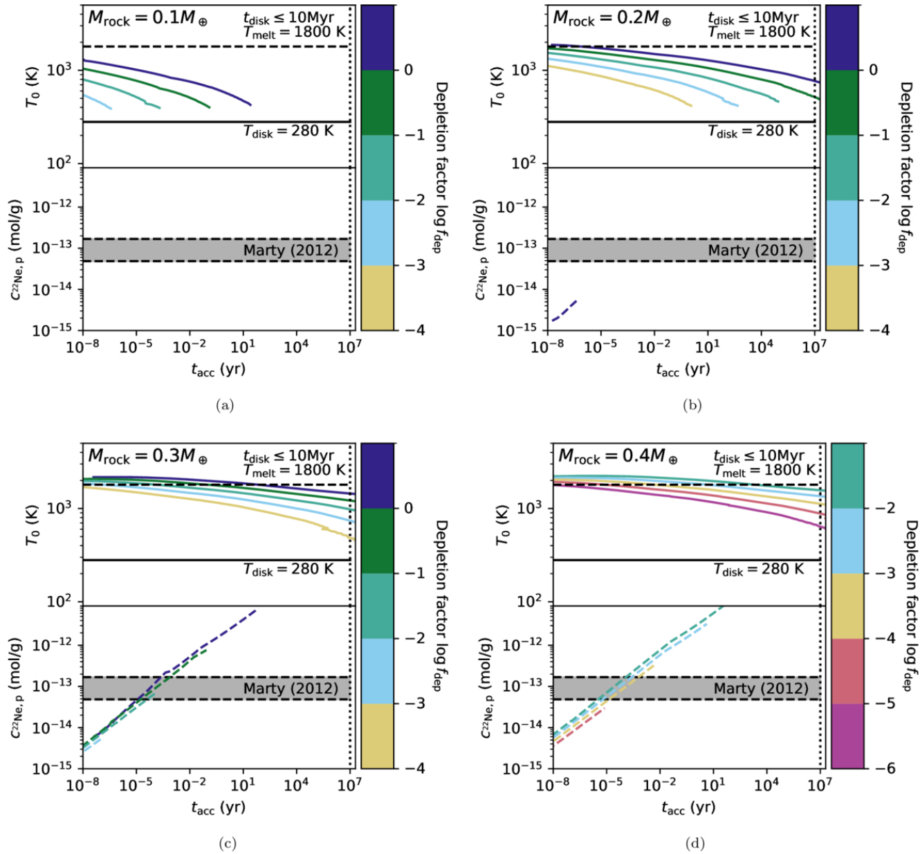
Figure 4. from Vincent Savignac and Eve J. Lee 2026 Planet. Sci. J. 7 doi:10.3847/PSJ/ae64f7 https://dx.doi.org/10.3847/PSJ/ae64f7 © 2026. The Author(s). Published by the American Astronomical Society.
