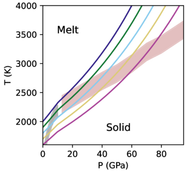
Figure 3. from Vincent Savignac and Eve J. Lee 2026 Planet. Sci. J. 7 doi:10.3847/PSJ/ae64f7 https://dx.doi.org/10.3847/PSJ/ae64f7 © 2026. The Author(s). Published by the American Astronomical Society.
