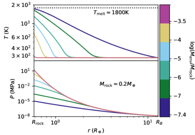
Figure 2. from Vincent Savignac and Eve J. Lee 2026 Planet. Sci. J. 7 doi:10.3847/PSJ/ae64f7 https://dx.doi.org/10.3847/PSJ/ae64f7 © 2026. The Author(s). Published by the American Astronomical Society.
