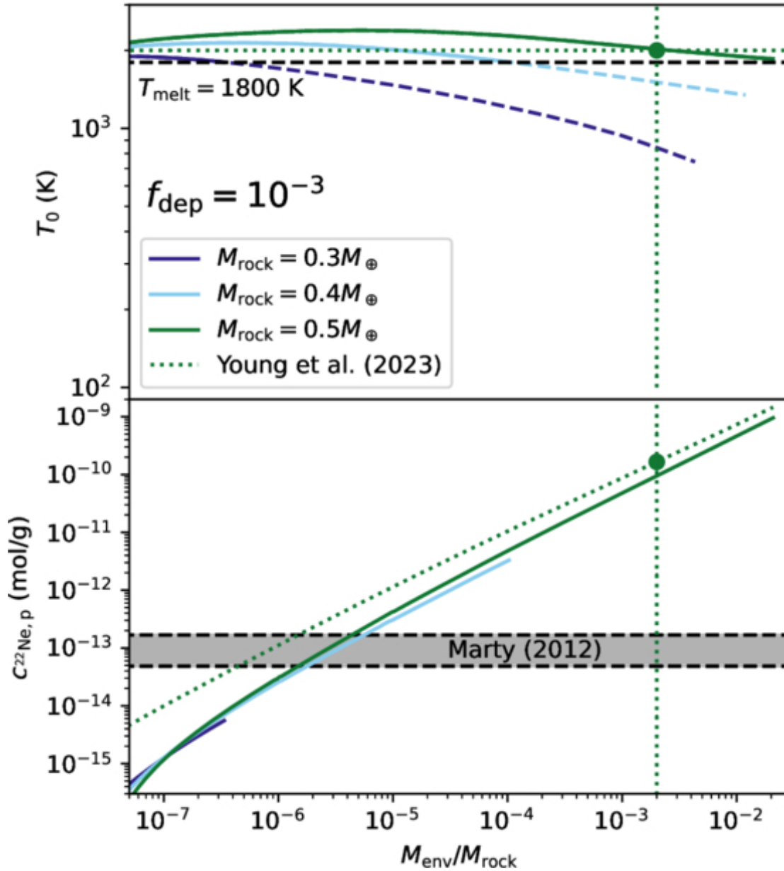
Figure 10. from Vincent Savignac and Eve J. Lee 2026 Planet. Sci. J. 7 doi:10.3847/PSJ/ae64f7 https://dx.doi.org/10.3847/PSJ/ae64f7 © 2026. The Author(s). Published by the American Astronomical Society.
