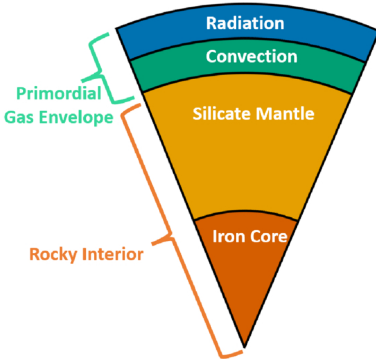
Figure 1. from Vincent Savignac and Eve J. Lee 2026 Planet. Sci. J. 7 doi:10.3847/PSJ/ae64f7 https://dx.doi.org/10.3847/PSJ/ae64f7 © 2026. The Author(s). Published by the American Astronomical Society.
