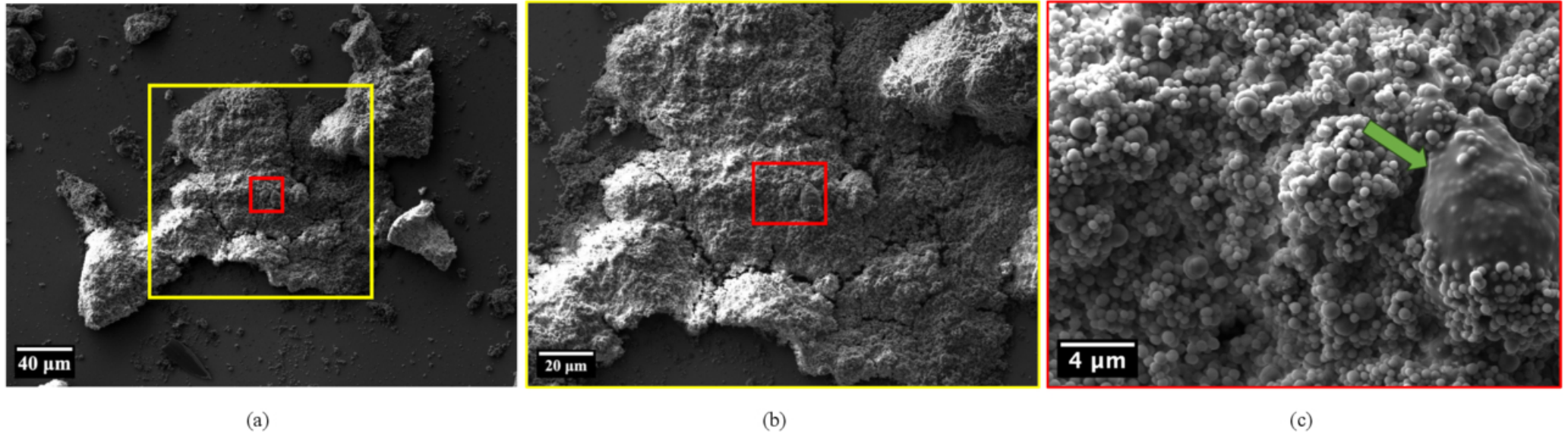
Figure 3. from Adis Husi et al 2026 Planet. Sci. J. 7 doi:10.3847/PSJ/ae63ca https://dx.doi.org/10.3847/PSJ/ae63ca © 2026. The Author(s). Published by the American Astronomical Society.
