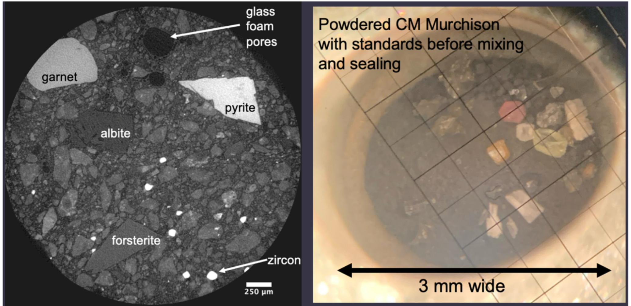
Figure B1. from Romy D. Hanna et al 2026 Planet. Sci. J. 7 doi:10.3847/PSJ/ae63c9 https://dx.doi.org/10.3847/PSJ/ae63c9 © 2026. The Author(s). Published by the American Astronomical Society.
