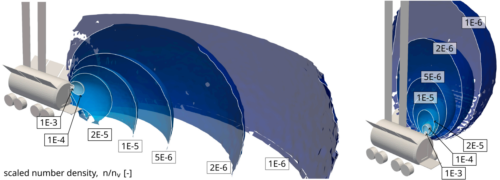
Figure 7. from S. Boccelli et al 2026 Planet. Sci. J. 7 doi:10.3847/PSJ/ae63c4 https://dx.doi.org/10.3847/PSJ/ae63c4 © 2026. The Author(s). Published by the American Astronomical Society.
