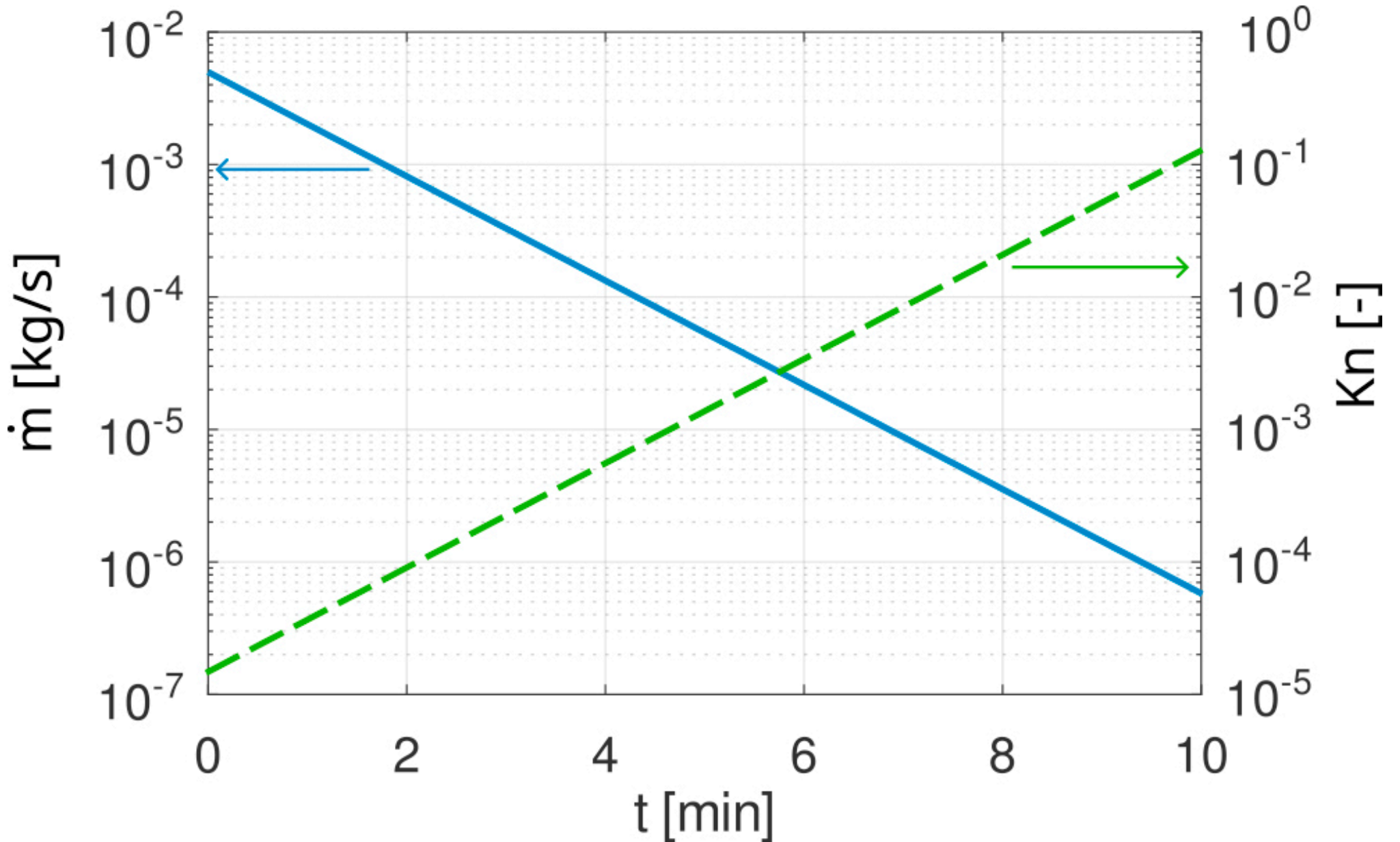
Figure 5. from S. Boccelli et al 2026 Planet. Sci. J. 7 doi:10.3847/PSJ/ae63c4 https://dx.doi.org/10.3847/PSJ/ae63c4 © 2026. The Author(s). Published by the American Astronomical Society.
